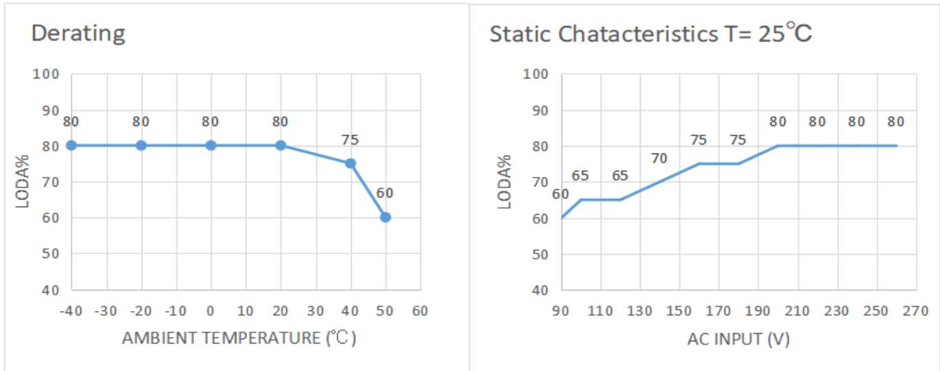
带载降额曲线: Load derating curve:
