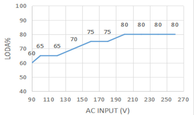
Static Characteristics T= 25°C
