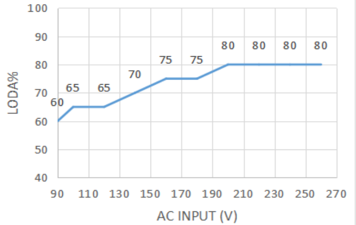
Static Characteristics T= 25°C
