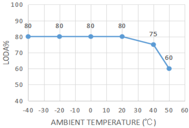
Derating
